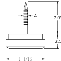
Heavy Duty Insulated Glides
