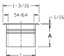
Post Hole Liners
