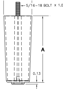
Plastic Leg w/bolt
