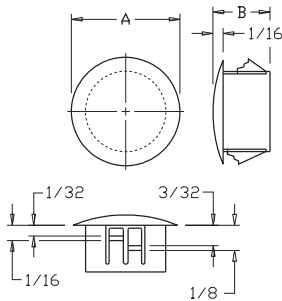
Nylon Hole Plugs
