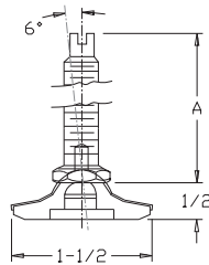
Swivel Adjustable Levelers
