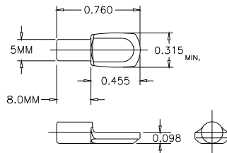
5mm x 8mm Peg
