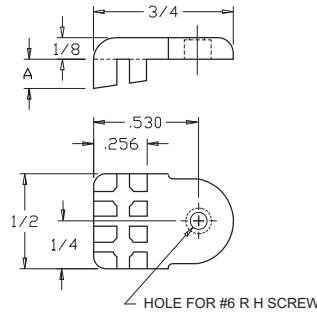
Tapered Pad Retainers
