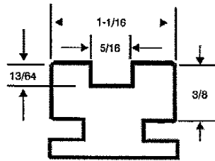
Wood Case Runner Dimensions* *(Wood Case Runner Not Included)
